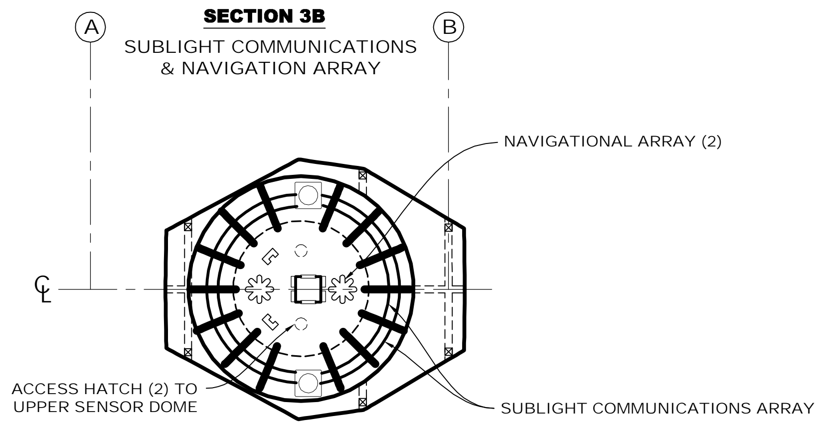
DECK 3 FORWARD
