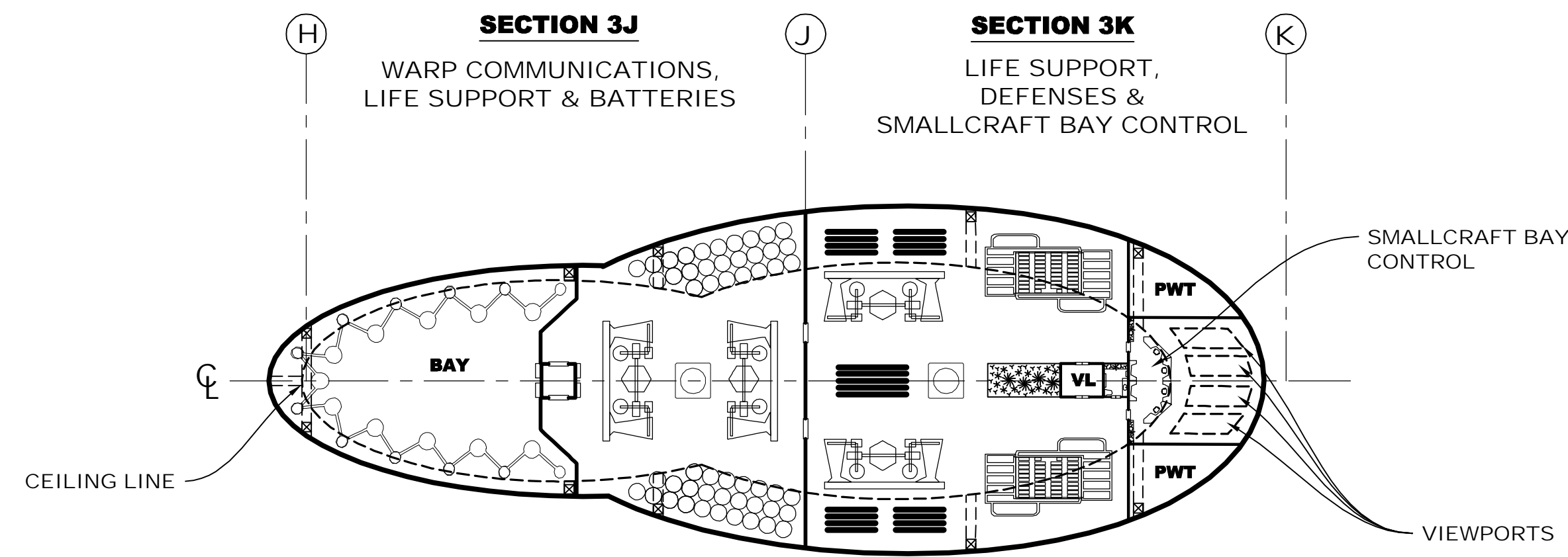
DECK 3 AFT
